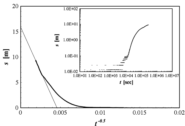
Figure 3. Asymptotic analysis of drawdown data from observation interval B13-2, with inset showing the double-logarithmic plot.
