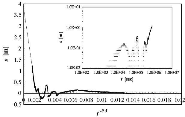
Figure 4. Asymptotic analysis of drawdown data from observation interval F22-2, with inset showing the double-logarithmic plot.
