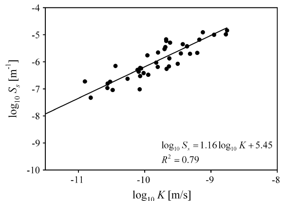
Figure 7. \log_{10}S_s vs. \log_{10}K with a linear model fit to the data set.
