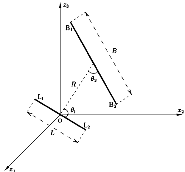
Figure 1. A schematic representation of a cross-hole injection test. The lengths of injection ( L_1L_2 ) and monitoring ( B_1B_2 ) intervals are L and B , respectively. The centroid of the former coincides with the origin of the coordinate system, while the centroid of the latter is located at the distance R away. The angles between the line connecting the two centroids and the injection and monitoring intervals are \theta_1 and \theta_2 , respectively.
