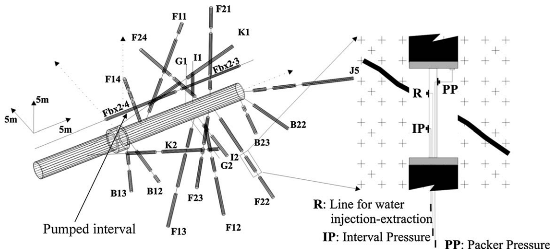
Figure 2. View of the 23 control boreholes in the test area. They are divided into intervals by means of inflatable packers. Each interval is equipped with a pressure intake, which is connected to an outer pressure transducer, and with a water recirculation intake for performing hydrochemical sampling and hydraulic tests. This leads to a total of 64 observation points (modified after Martínez-Landa and Carrera 2005).
