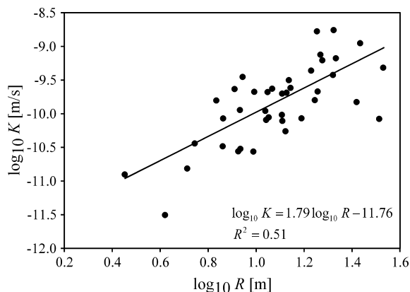
Figure 5. \log_{10}K vs. \log_{10}R with a linear model fit to the data set.
